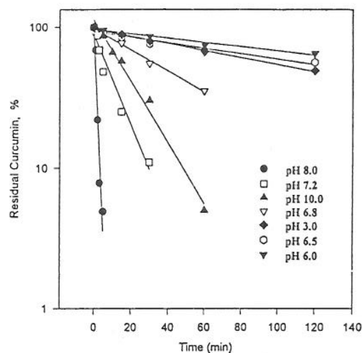
Figure 1. Apparent first-order plots for the degradation of curcumin at various pH values. The data are normalized to a value of 100 at zero time. Points represent the experimental data and the solid lines were drawn using linear least-squares regression analysis.
